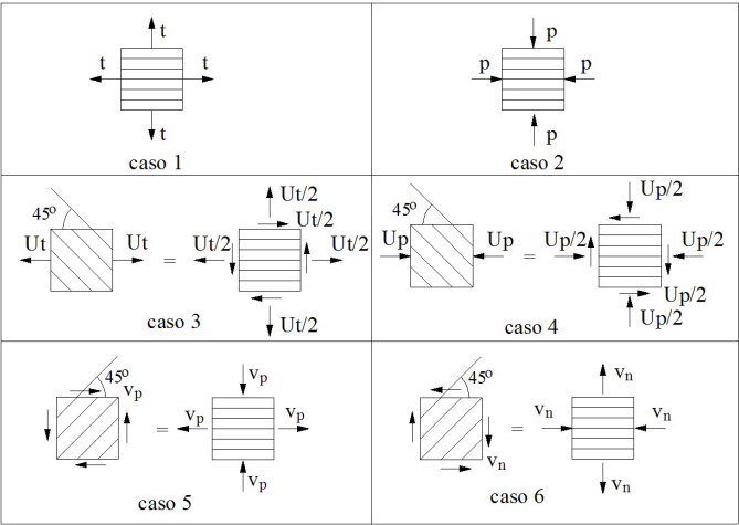
Fig. 1: – Biaxial and uniaxial tests (cases 1 to 6).
