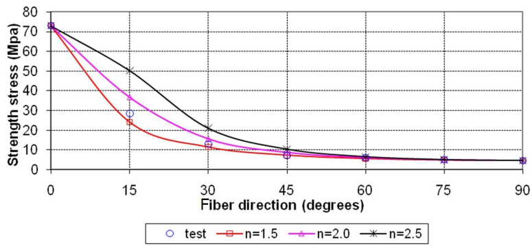
Fig. 5: Comparison between Hankinson's formula and data from tensile tests.
