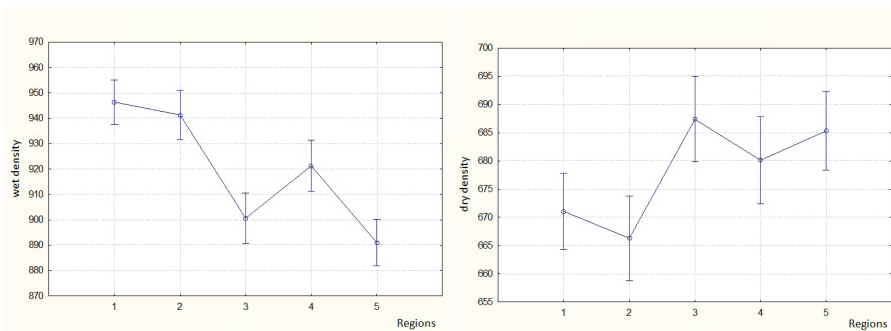
Fig. 3: Wet (left) and dry (right) wood density of Hornbeam in different regions (1: Szigetvár; 2: Pécsvárad; 3: Sásd; 4: Sellye; 5: Árpádtető) Vertical bars show the 0.95 confidence intervals.
