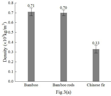
Fig. 3a: Comparison of properties of bamboo, bamboo rods and Chinese fir. Comparison of density. Fig. 3b: Comparison of properties of bamboo, bamboo rods and Chinese fir. Comparison of compressive strength and modulus.
