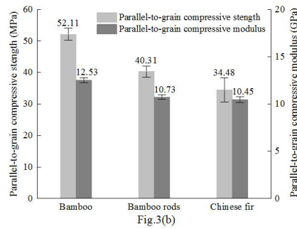
Fig. 3a: Comparison of properties of bamboo, bamboo rods and Chinese fir. Comparison of density. Fig. 3b: Comparison of properties of bamboo, bamboo rods and Chinese fir. Comparison of compressive strength and modulus.
